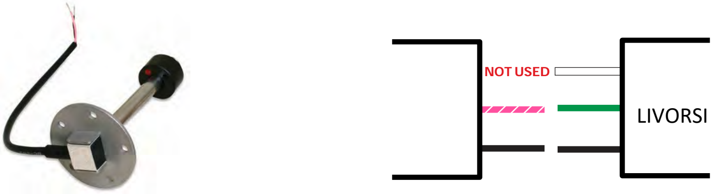
2 WIRE FUEL/WATER SENDER (ANALOG)
