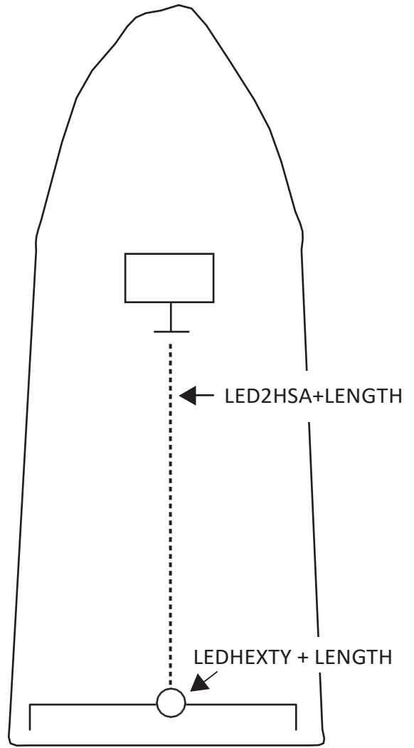
LEDHEXTY + LENGTH Designed to be installed in center of boat
