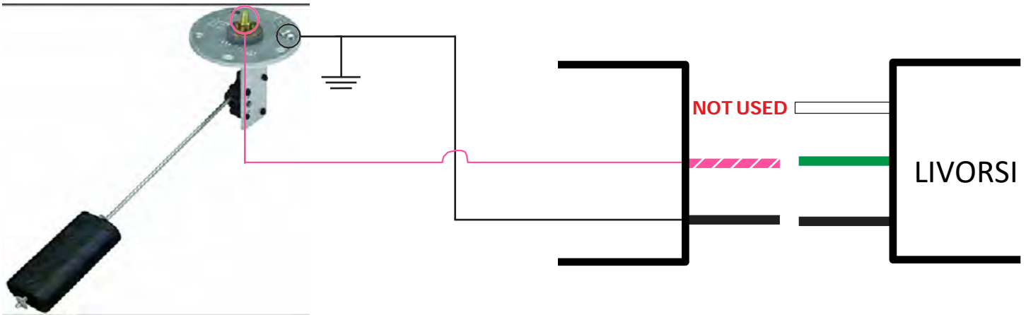
2 WIRE FUEL/WATER SENDER (ANALOG)
