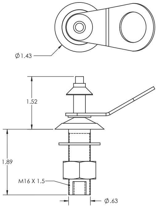
Fender Cleat- QPC
