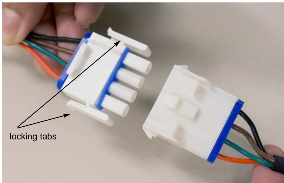
Female connector from the master harness
